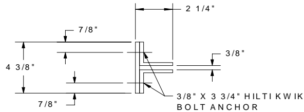
SURFACE GUIDE DETAIL
