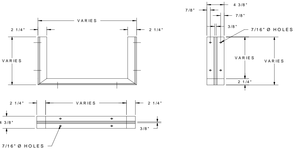
SURFACE MOUNT GUIDE DETAIL
